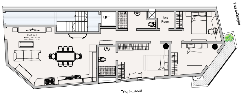
GROUND FLOOR AS PROPOSED Scale 1:100
