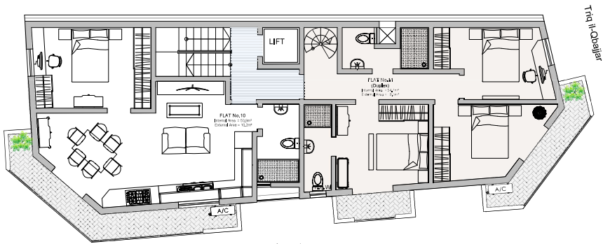
Triq il-Luzzu FIFTH FLOOR AS PROPOSED Scale 1:100
