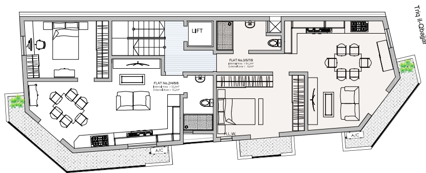
FIRST, SECOND THIRD & FOURTH FLOORS AS PROPOSED
