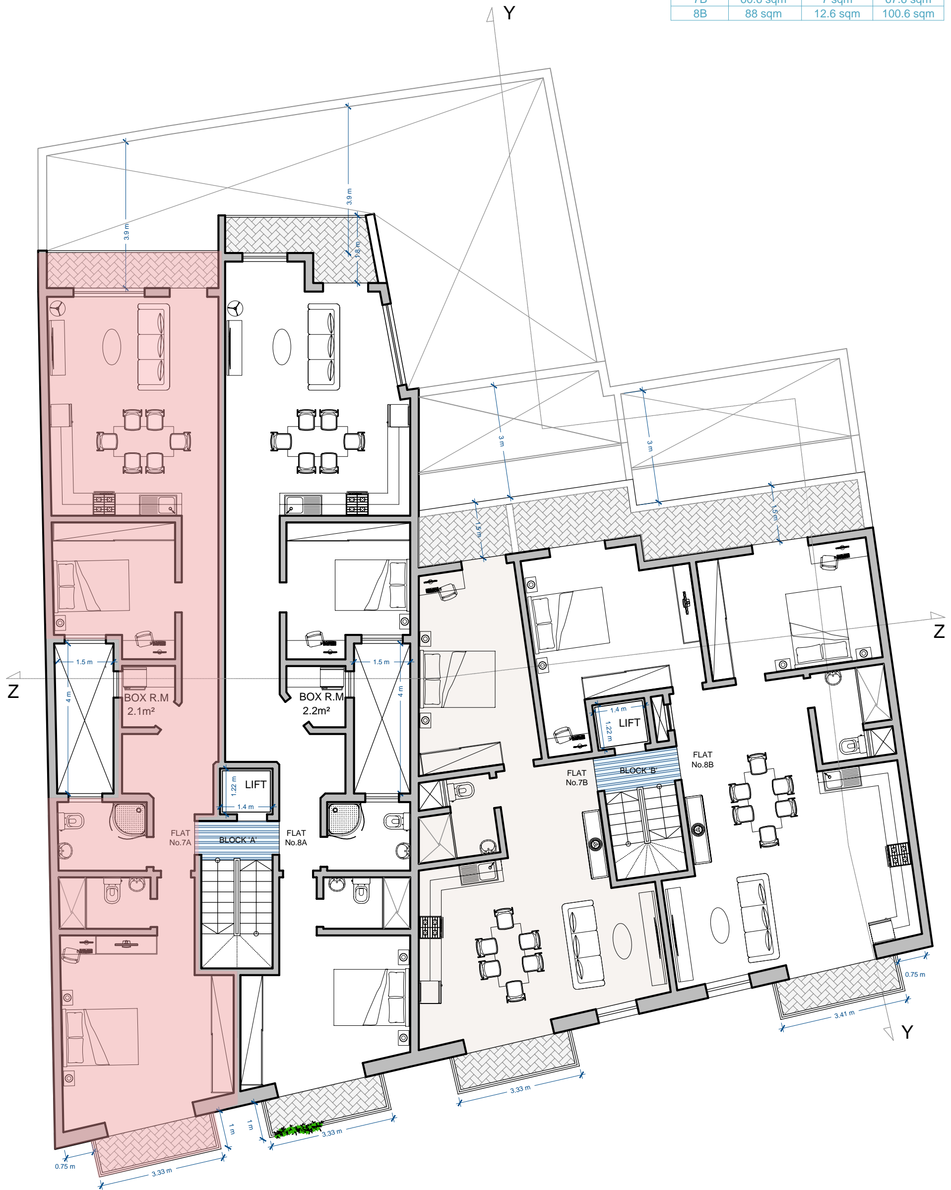
THIRD FLOOR PROPOSED Scale 1:100
