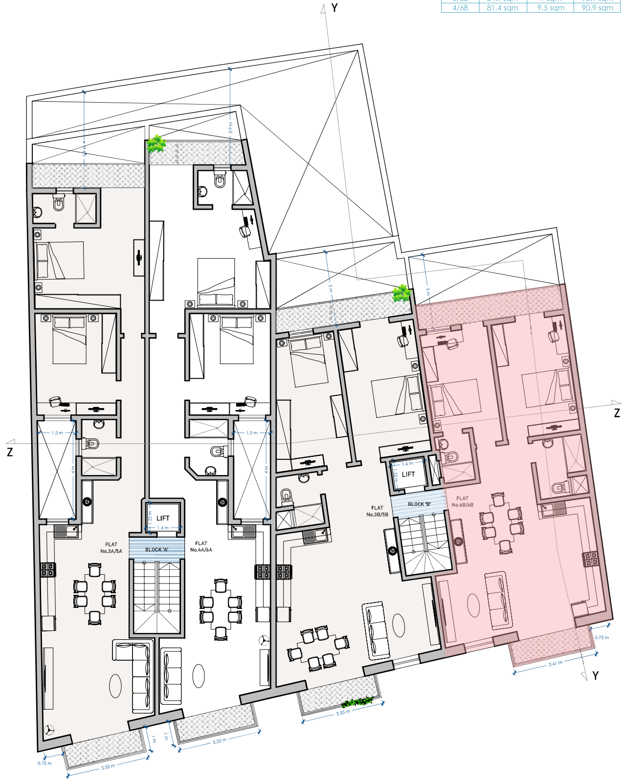
FIRST & SECOND FLOORS PROPOSED Scale 1:100
