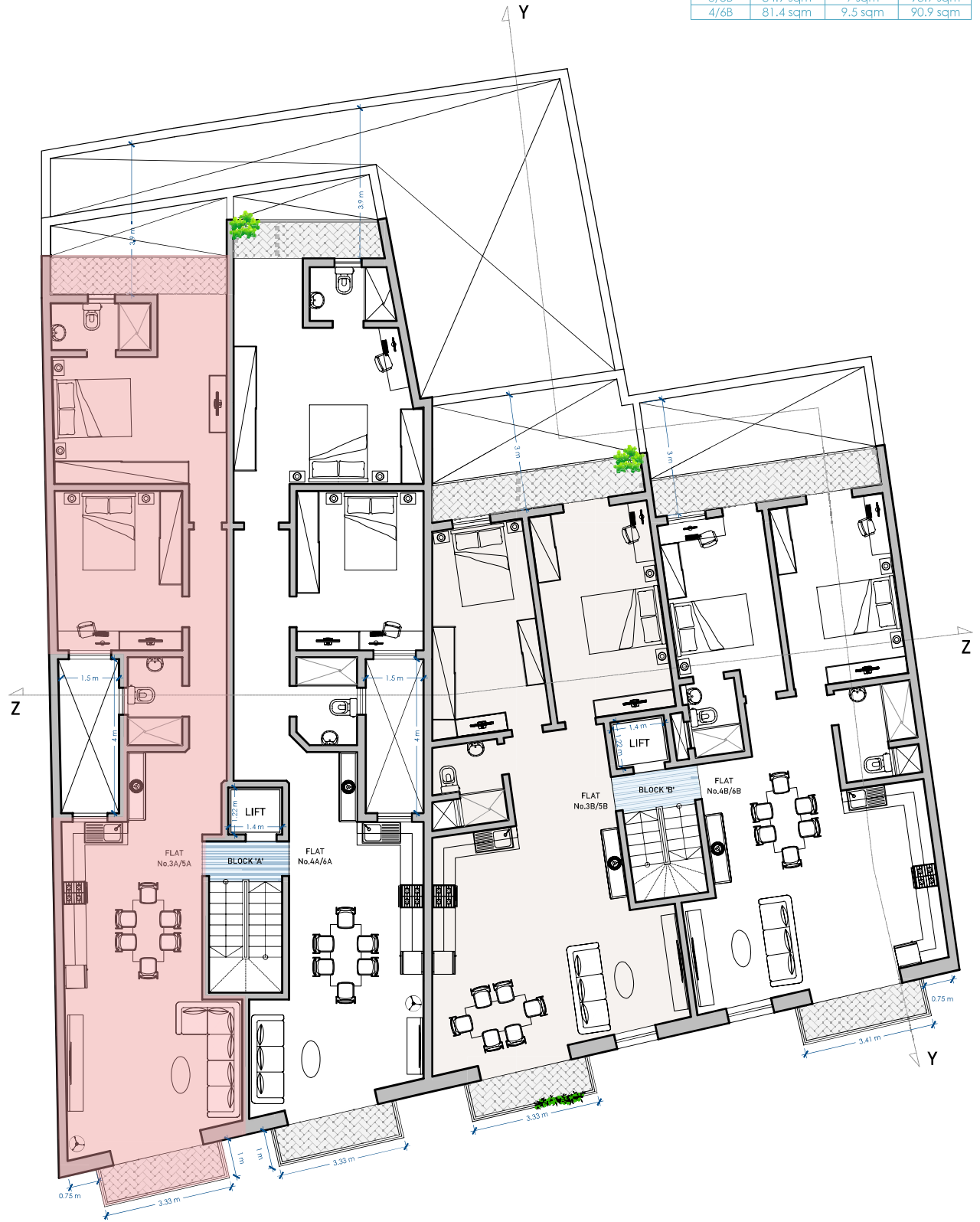
FIRST & SECOND FLOORS PROPOSED Scale 1:100
