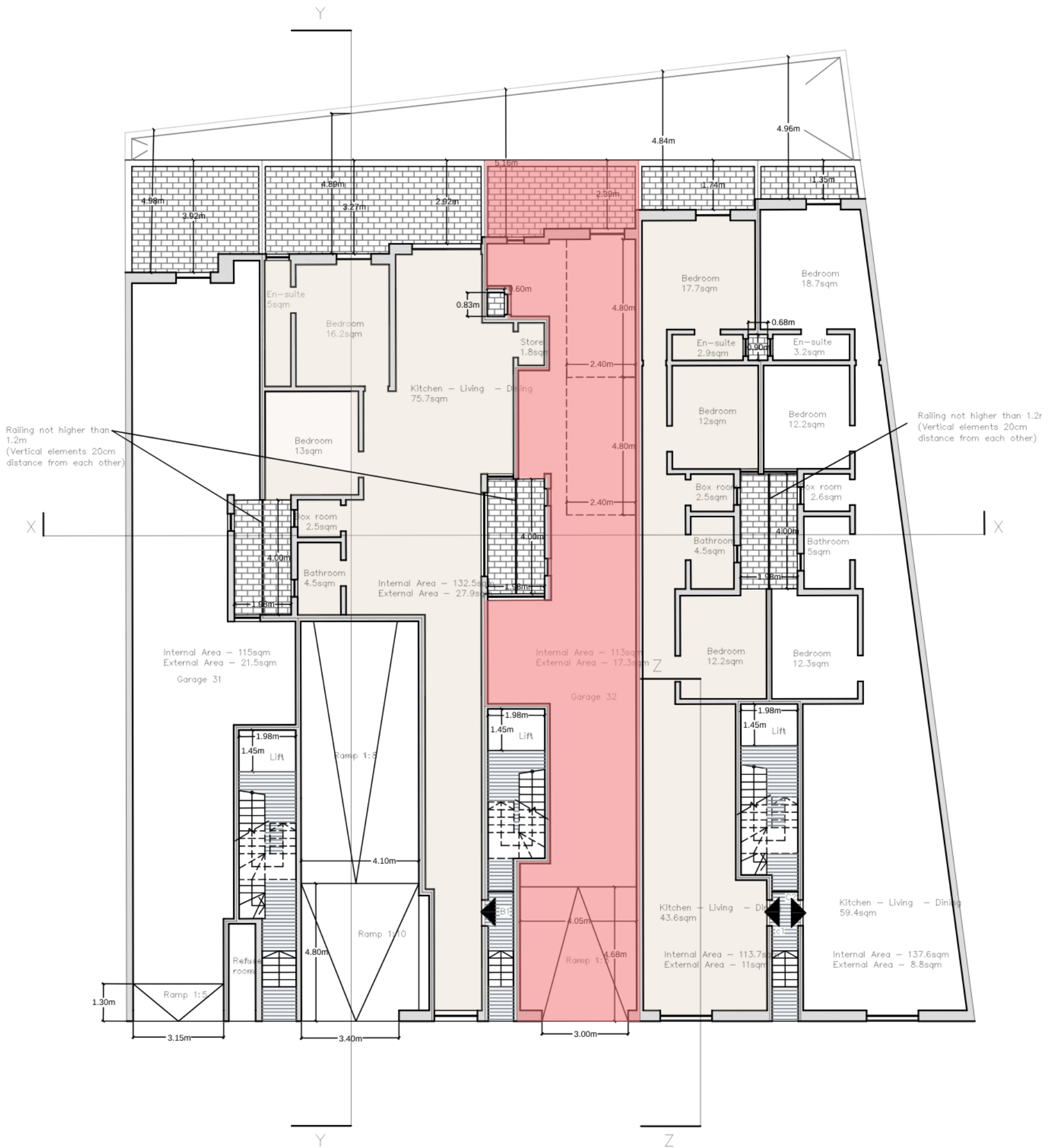
GROUND FLOOR PROPOSED SCALE 1:150
